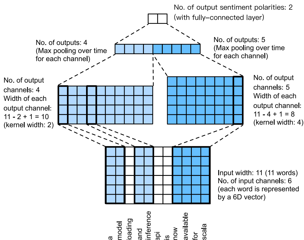
Fig. 15.3.5: TextCNN design.
